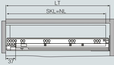
塑料后连接件 Plastic rear mounting bracket
