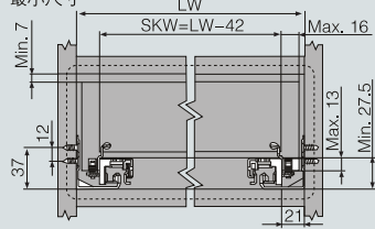
钢后连接件 Steel rear mounting bracket
