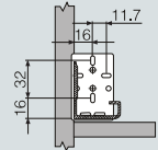
钢后连接件 Steel rear mounting bracket
