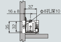
塑料后连接件 Plastic rear mounting bracket
